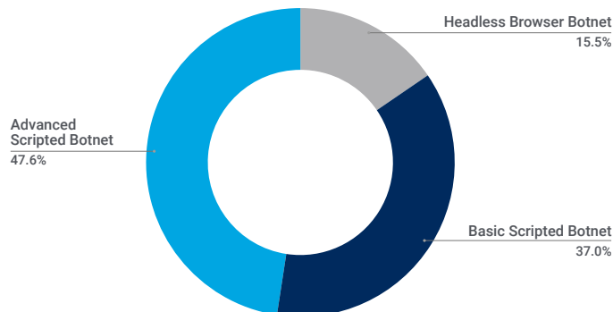
Fig. 9: Bad bots traffic distribution based on their sophistication (totals do not sum to 100% due to rounding)
