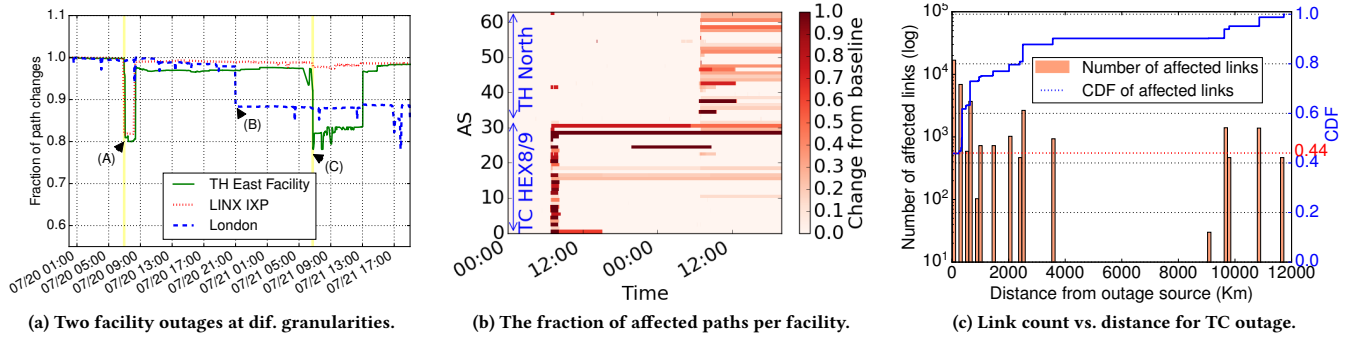
Figure 9: Two outages at different colocation facilities in London (TC HEX8/9 and TH North) at July 20 & 21, 2016.
