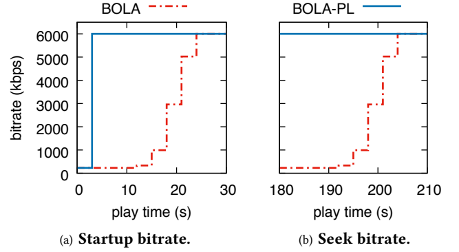
Figure 6: Bitrate of the video playout as a function of the video play time. BOLA with the placeholder algorithm (BOLA-PL) reacts more quickly by reaching the highest sustainable bitrate within a much shorter period of time after a startup or a seek than BOLA alone.
