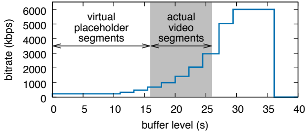
(b) BOLA-E bitrate decision function for a 10s buffer capacity after buffer expansion. While the video buffer is still limited to 10s of actual segments, the placeholder segments can slide the 10s window, allowing more separation between thresholds.
