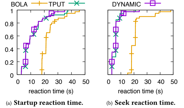
Figure 10: CDF of the reaction time for BOLA versus THROUGHPUT versus DYNAMIC during startup and seek for 40 4G network traces. THROUGHPUT and DYNAMIC react much more quickly and stream at the highest sustainable bitrate sooner than BOLA.
