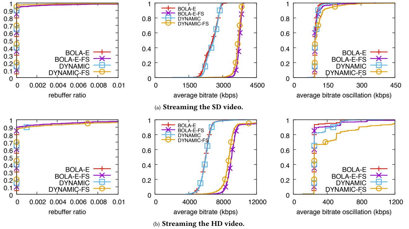
Figure 13: CDF of QoE metrics with and without FAST SWITCHING using a 25s buffer.
