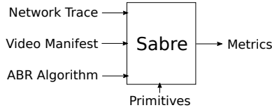
Figure 3: Sabre: Inputs, Outputs, and Primitives.
