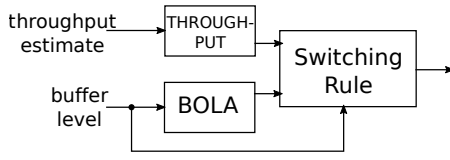
Figure 9: The DYNAMIC algorithm combines BOLA and THROUGHPUT.
