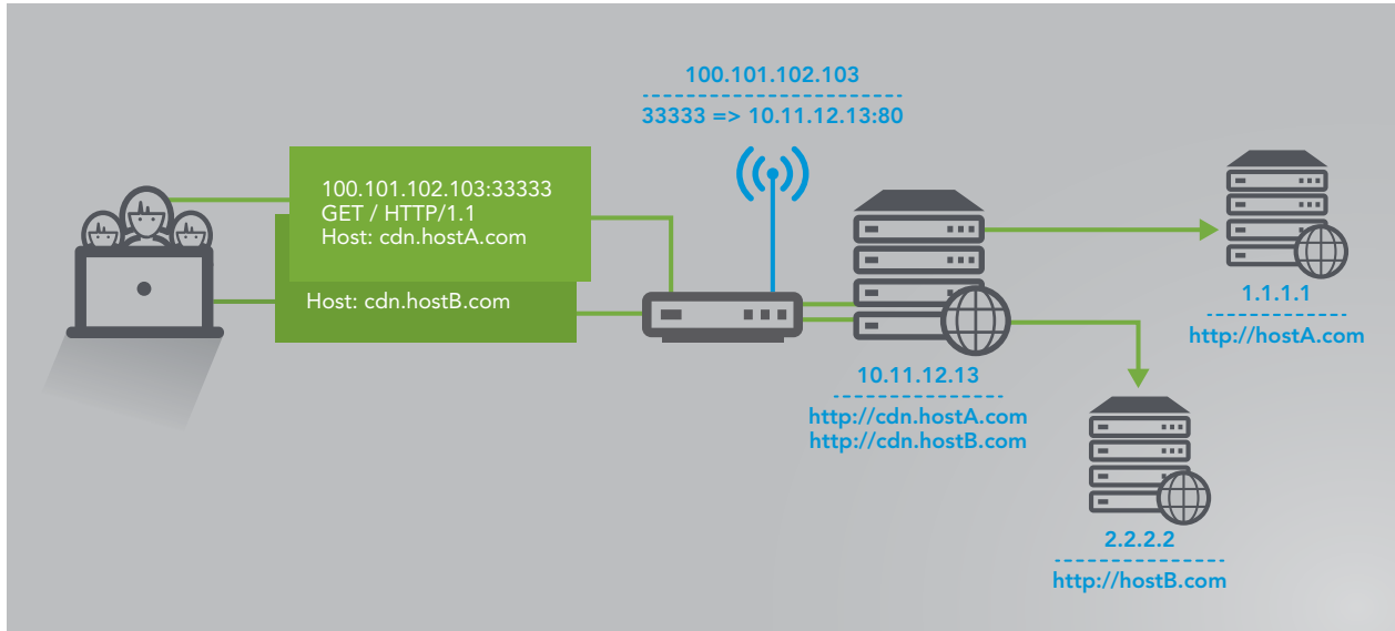
Figure 14: Virtual Hosts/Domain fronting example with UPnP injected proxy diagram
