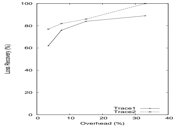
Fig. 6. Overhead and recovery rates of parity scheme across multiple streams.
