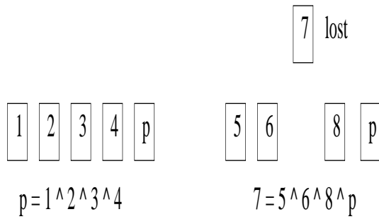
Fig. 3. Parity scheme across a single stream.
