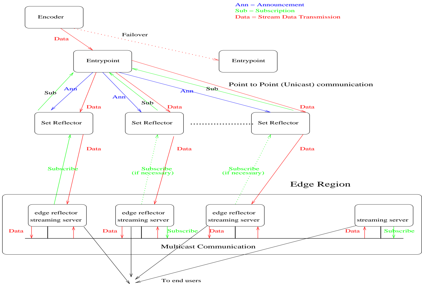
Fig. 1. High level diagram of a streaming CDN
