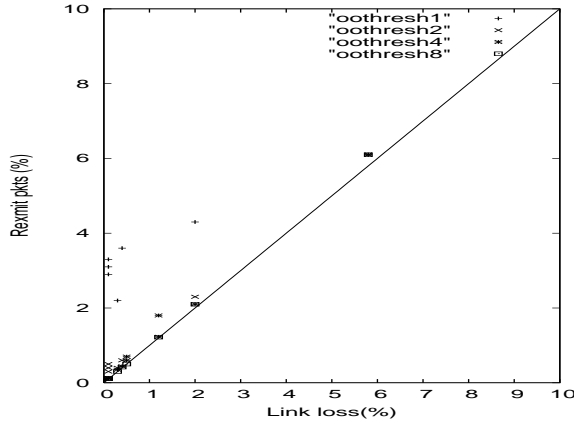
Fig. 8. Retransmit overhead as function of packet loss for different out of order tolerance thresholds.
